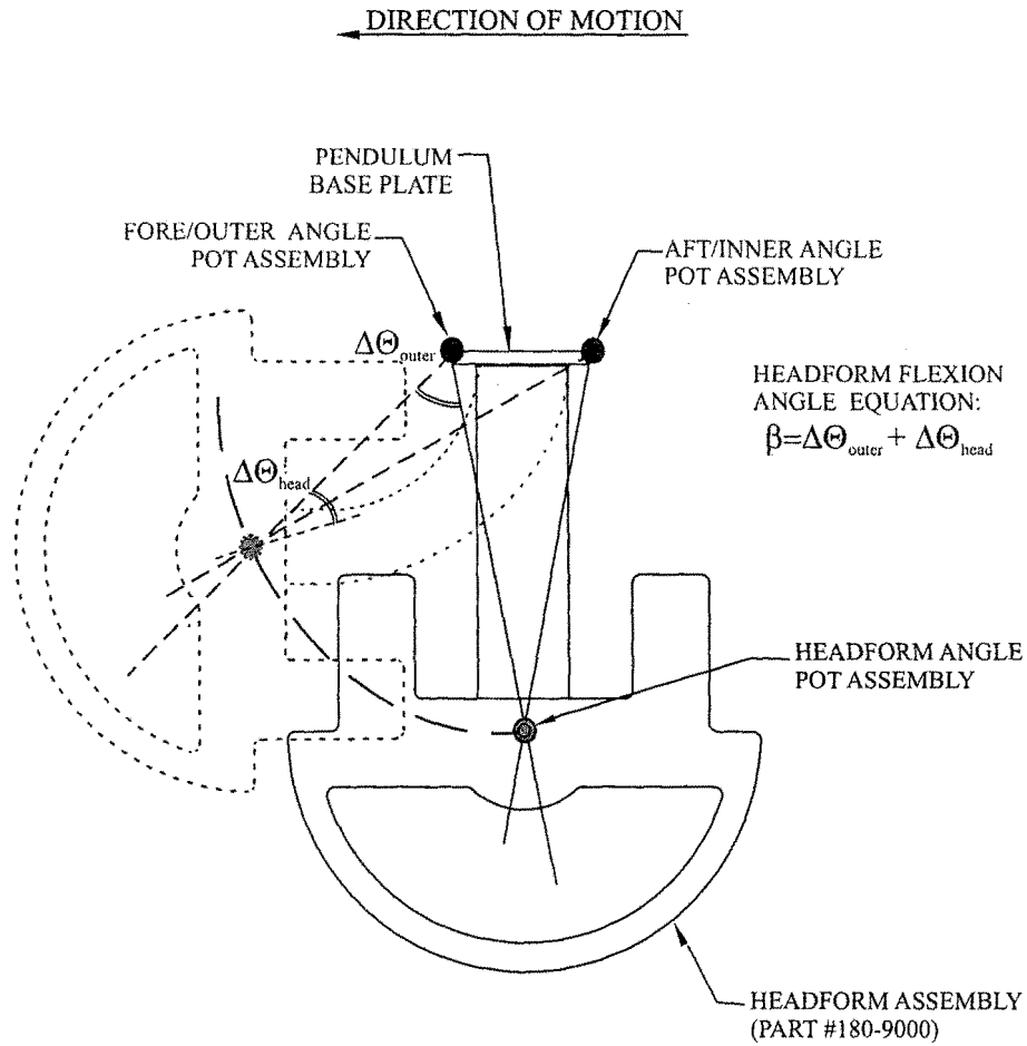
Figure V2-C ANGLE MEASUREMENTS WITH HEADFORM SET-UP
