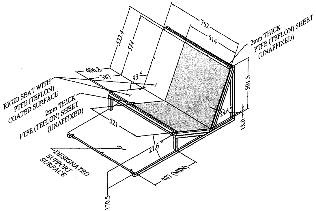
FIGURE V4 CERTIFICATION BENCH
